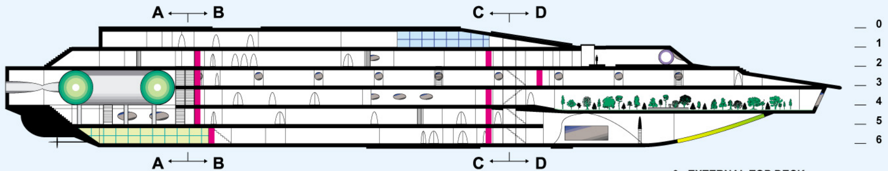
STARBOARD CUTAWAY PROFILE
