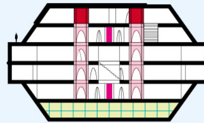
VIEW B-B
